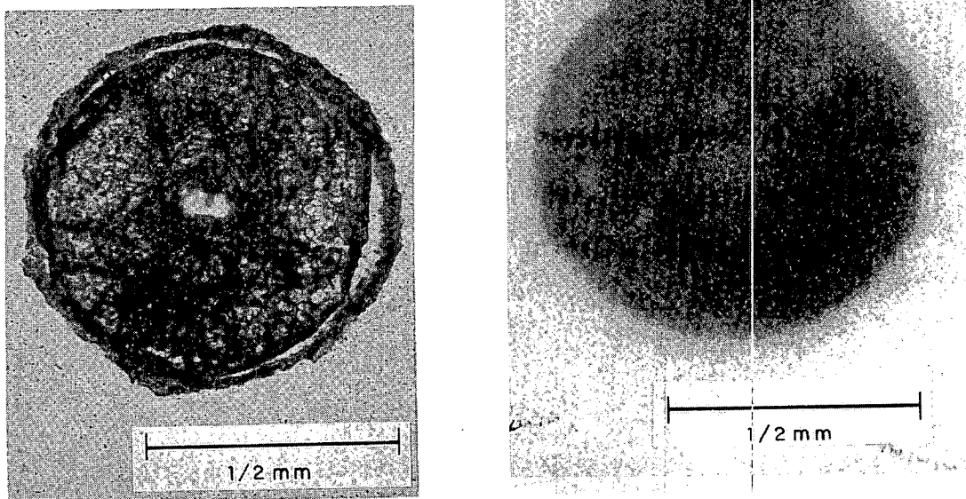
Fig. 3. Photograph (left) and autoradiograph (right) of a thin section of a spherical particle from a ground surface shot at Eniwetok. The radioactivity is uniformly distributed throughout the particle.
